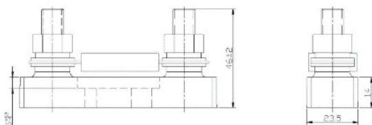
MEGA fuse
