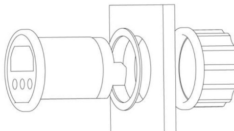
Mounting sequence
